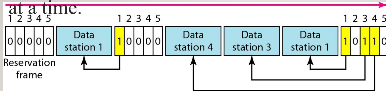
Figure 15 Reservation access method
