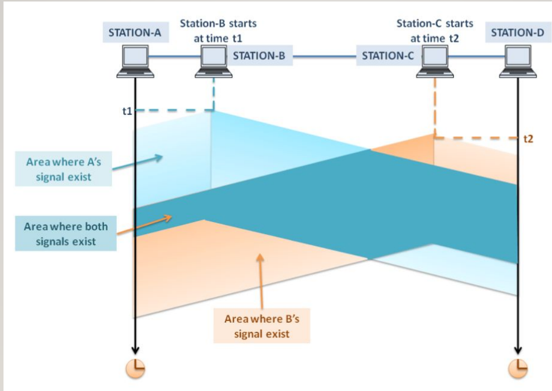
Figure 8 Space/time model of the collision in CSMA
