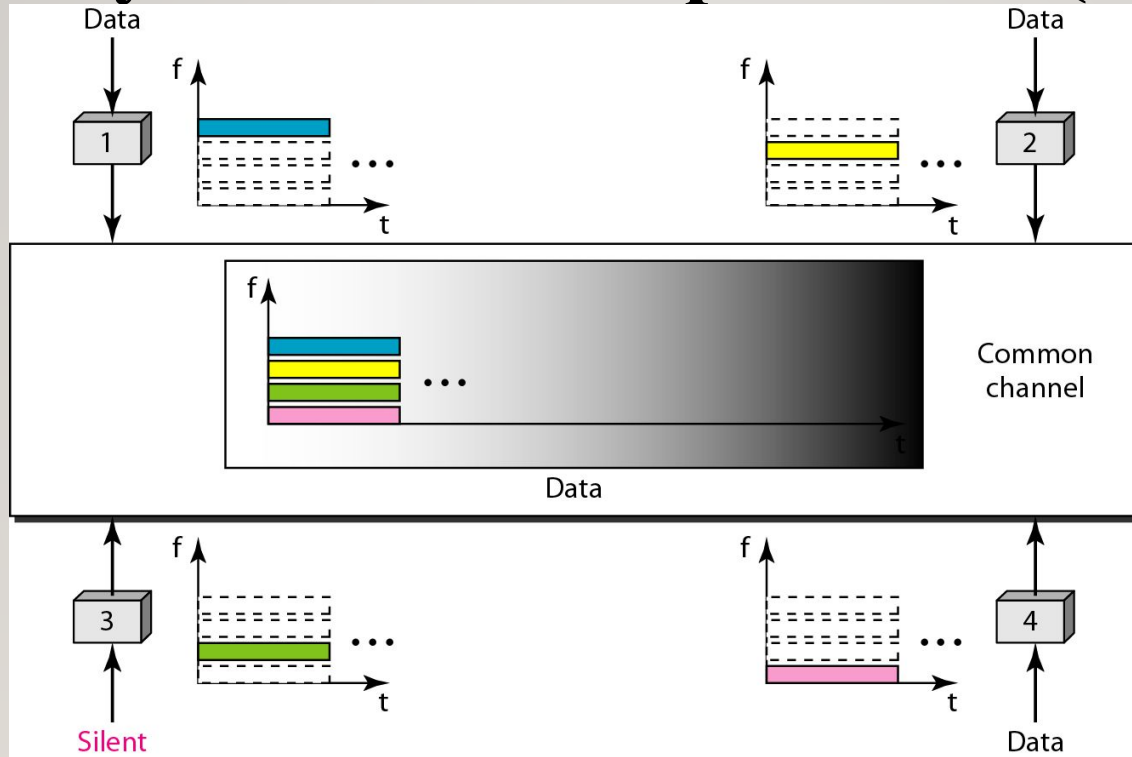
Figure 19 Frequency-division multiple access (FDMA)
