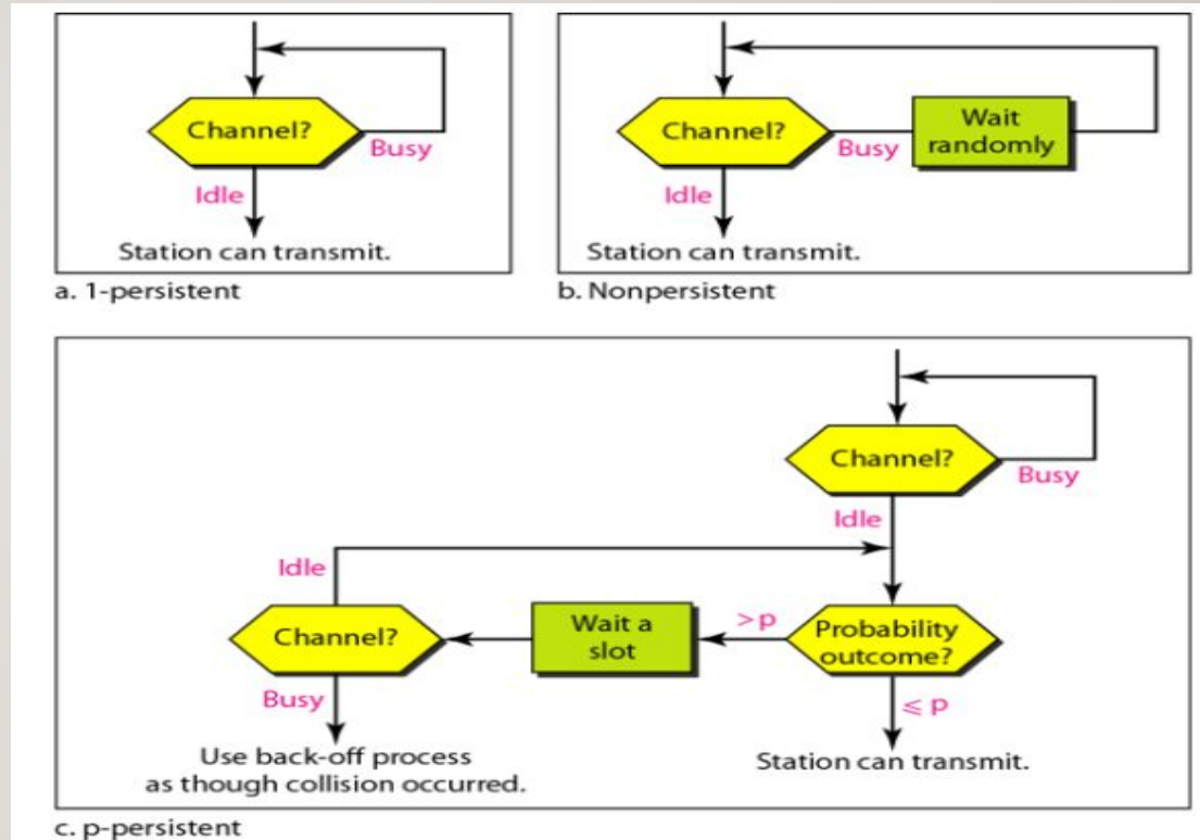
Figure 7 Flow chart of CSMA persistent methods
