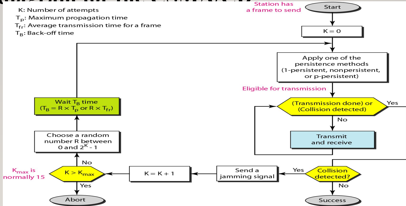
Figure 11 Flow diagram for the CSMA/CD
