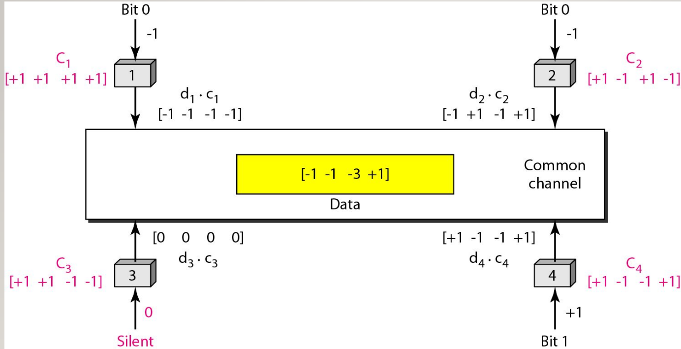
Figure24 Sharing channel in CDMA
