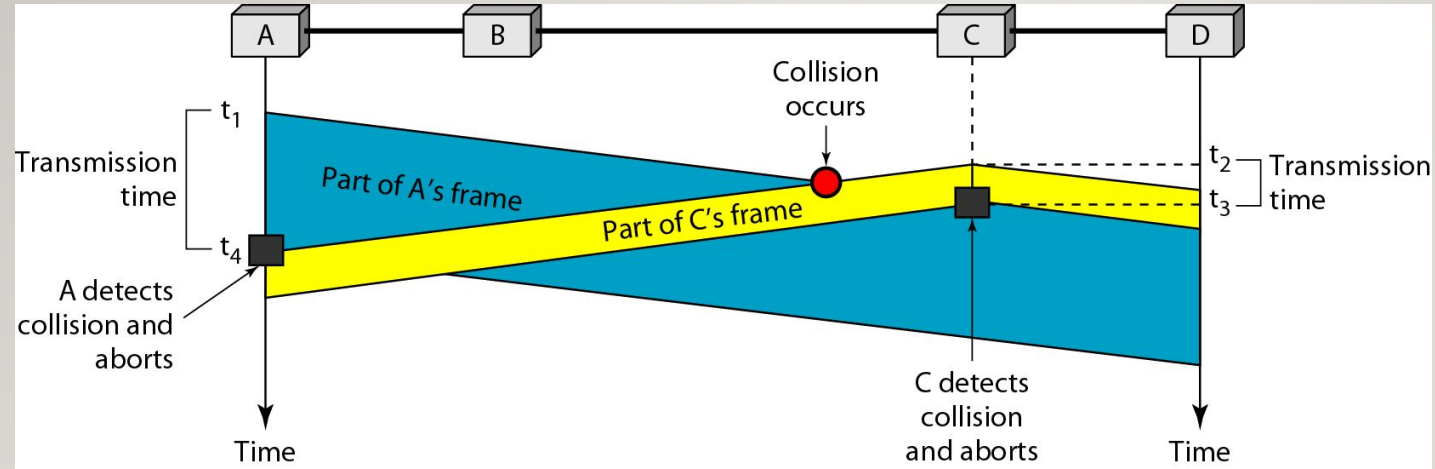
Figure 10 Collision and abortion in CSMA/CD
