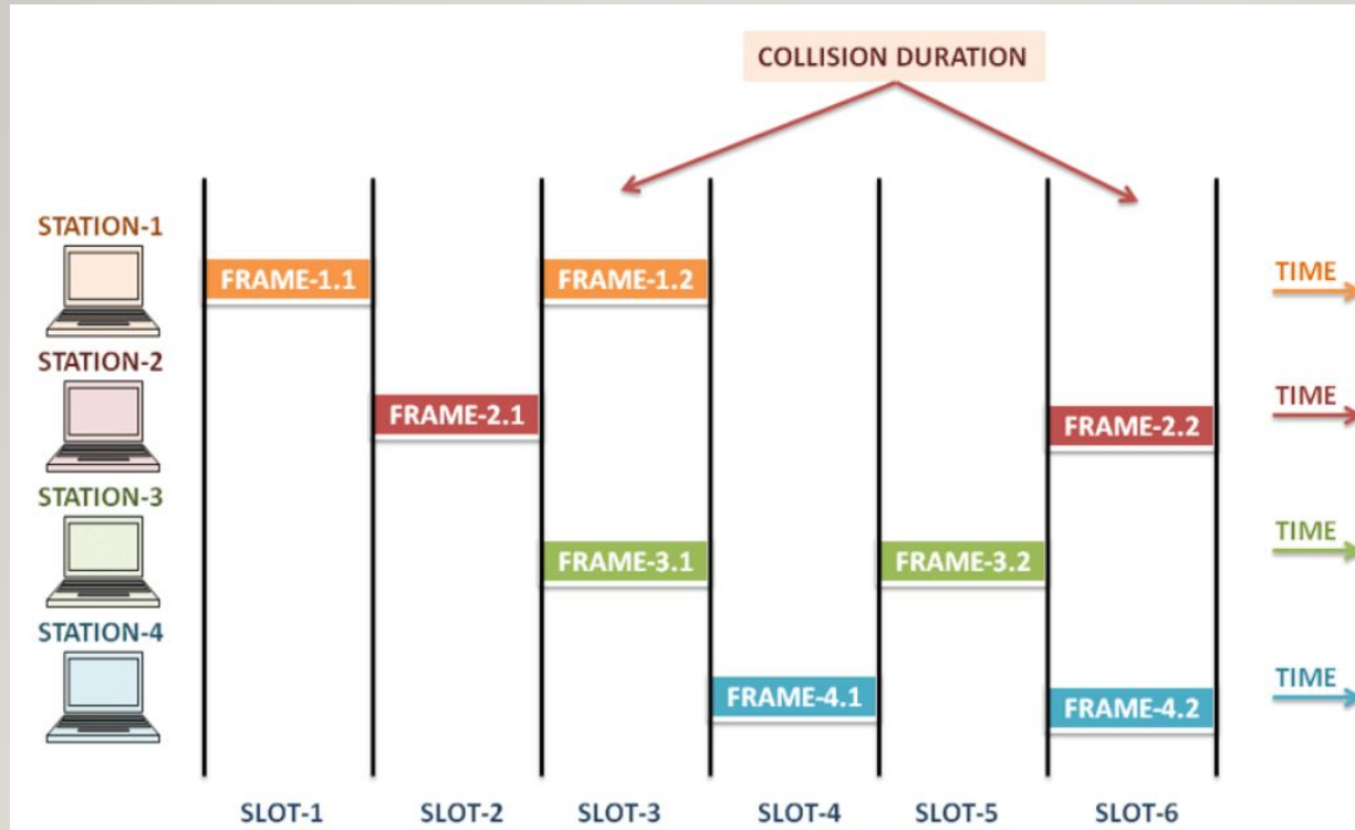
Figure 5 Frames in a slotted ALOHA network
