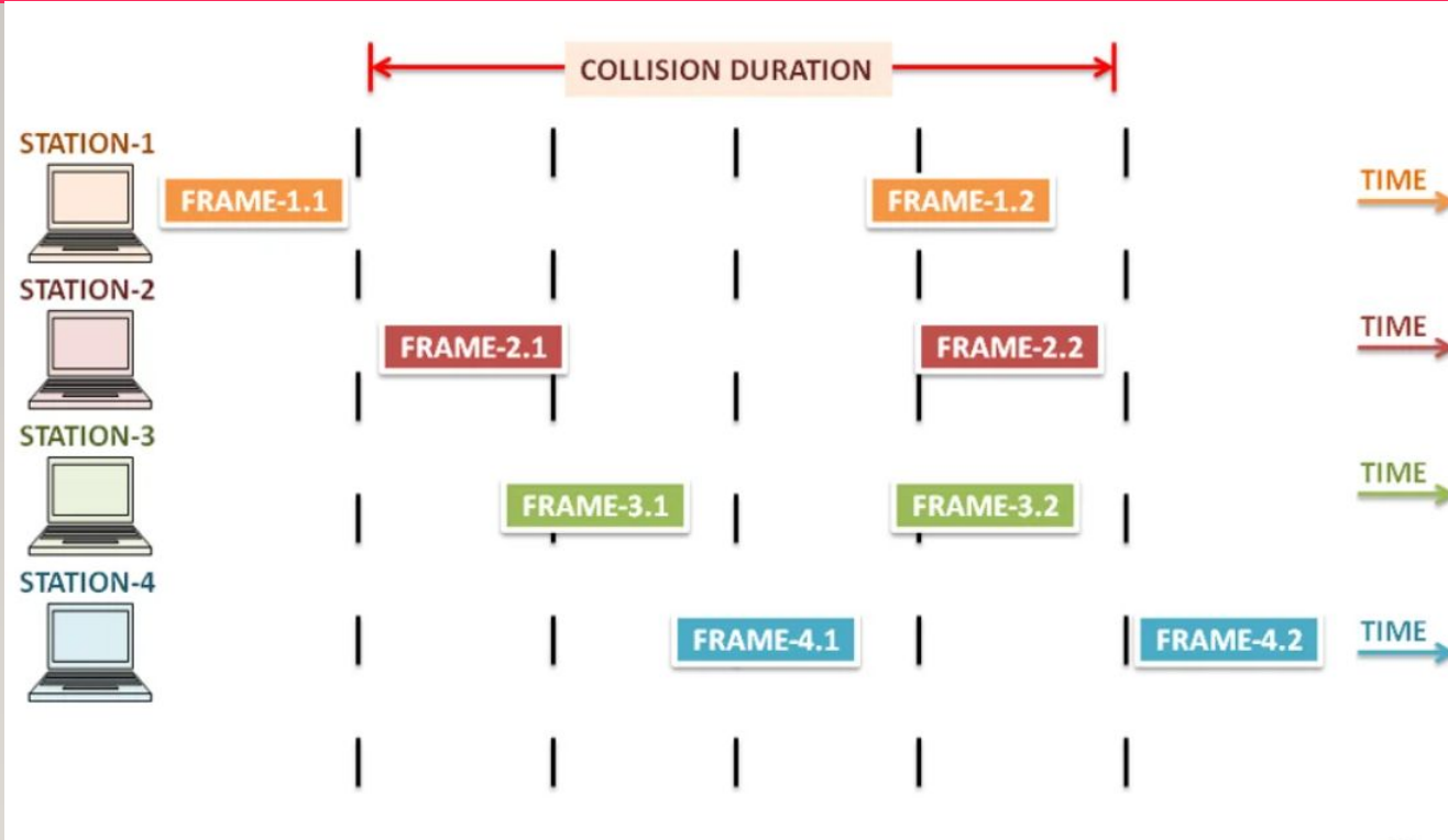
Figure 3 Procedure for pure ALOHA protocol
