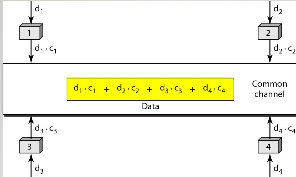
Figure 21 Simple idea of communication with code
